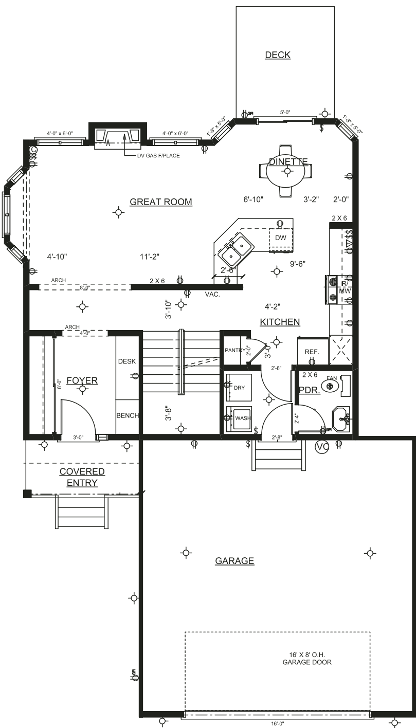
MAIN FLOOR PLAN 802 SQ. FT.
