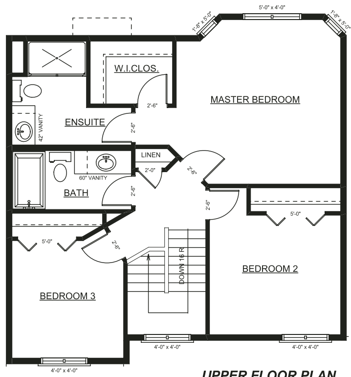
UPPER FLOOR PLAN 735 SQ. FT.
